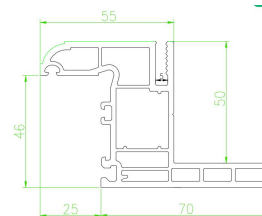
60H 转换框 SPC60-05H
