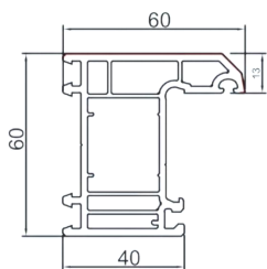
60K内平开框 SPKB6010B
