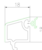
60 双压(A) PC60SYA
