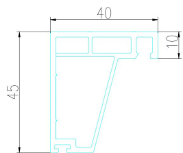
60 平开纱扇 PC60SS
