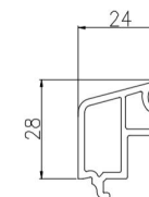
65 框双玻压条 SPC65K-02-02
