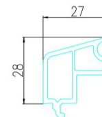
65 框双玻压条 SPC65K-02-01
