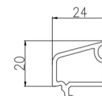
65 扇双玻压条 SPC65K-02-05
